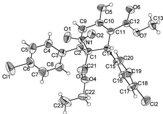
Figure 2. The molecular structure of 14a .
