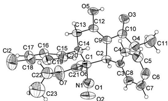
Figure 3. The molecular structure of 15a .
