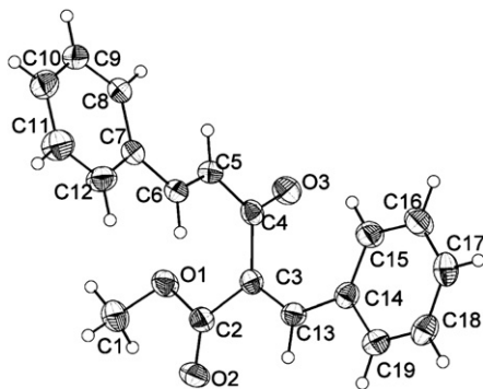
Figure 1. The molecular structure of 12b .
